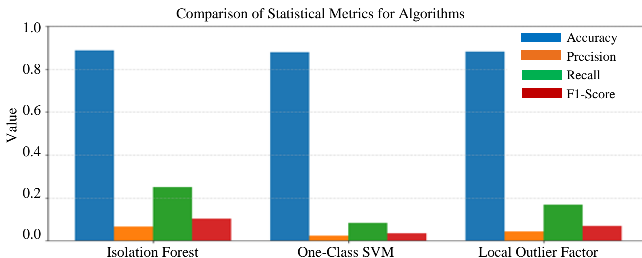
Fig. 2. Comparison chart of three algorithms
